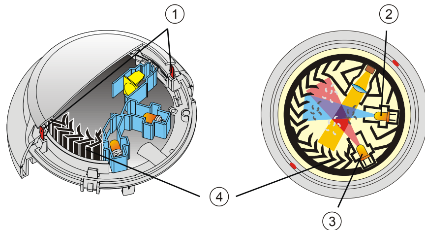
Figure 3: Fire detector structure
